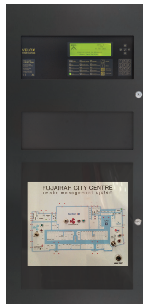
FIRE ALARM PANEL WITH SMOKE MANAGEMENT SYSTEM
